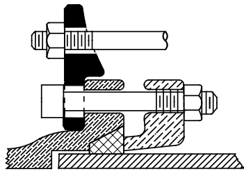
SDR 26 INSTALLATION
